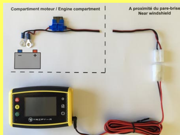
Porte fusible automobile / Automotive fuse holder
